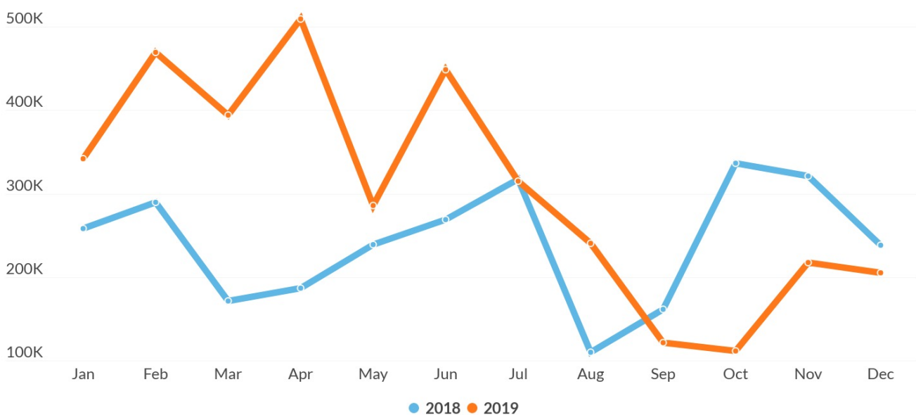
Encrypted Malware
